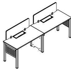
Linear Non-Sharing 2-PAX Cluster with Side Modesty & Straight Metal Legs
