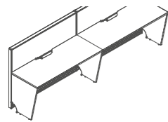
Non-sharing 2-Pax Cluster With Laminate Gable End
