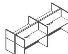
Sharing 4-Pax Cluster With 30mm Transform Panel
